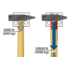
Tightening force
